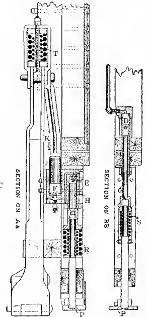
Fig. 2353. Section of Center Buffer. Fig. 2354. Section of Side Buffer.
